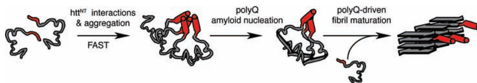
Figure 8. Schematic model of the htt NT -initiated aggregation process. (a) In solution, the monomeric species lacks a well-defined structure. The htt NT segment may have some helical propensity, but appears to lack a stable \alpha -helical structure. (b) The htt NT segment initiates the aggregation process, mediated by htt NT –htt NT interactions resulting in oligomeric species featuring substantial helicity. (c) This leads to a much-increased local polyQ concentration and permits the formation of the amyloid core, involving the generation of \beta -sheet secondary structure within the polyQ stretch. (d) Upon maturation, a highly rigid and dehydrated amyloid core (consisting of polyQ) is decorated with N-terminal residues 4–11 persisting in an \alpha -helix that is relatively mobile and solvent exposed. Not shown is the polyPro domain that forms an immobilized PPII helix in the mature fibrils.
