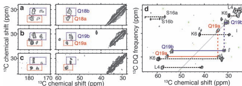
Figure 4. Doubling and similarity of glutamine resonances. (a, b) 2D ^{13}\text{C} – ^{13}\text{C} DARR spectral regions highlighting the Gln18 and Gln19 resonances in \text{htt}^{\text{NT}}\text{Q}_{30}\text{P}_{10}\text{K}_2 samples p2 and p3. For each residue we observe two distinct sets of resonances, marked as “a” (red) and “b” (blue). The cross-peak patterns suggest nearly identical chemical shifts for the C\beta and C\gamma sites in each case. (c) shows the virtually identical chemical shifts of a singly labeled glutamine within \text{K}_2\text{Q}_{30}\text{K}_2 fibrils ( U\text{-}^{13}\text{C},^{15}\text{N} -Gln6, the fourth residue within polyQ). (d) 2D ^{13}\text{C} – ^{13}\text{C} SQ–DQ spectrum for sample p3 (using 1.5 ms SPC ^3 mixing at 12 kHz MAS and \omega_{0\text{H}}/2\pi = 600 MHz), showing analogously color-coded Gln19 cross-peaks. Doubling appears specific to the \beta -sheet structure: singular sets of resonances are observed for helical residues (e.g., Leu4); doubling can also be seen for Ser16.
