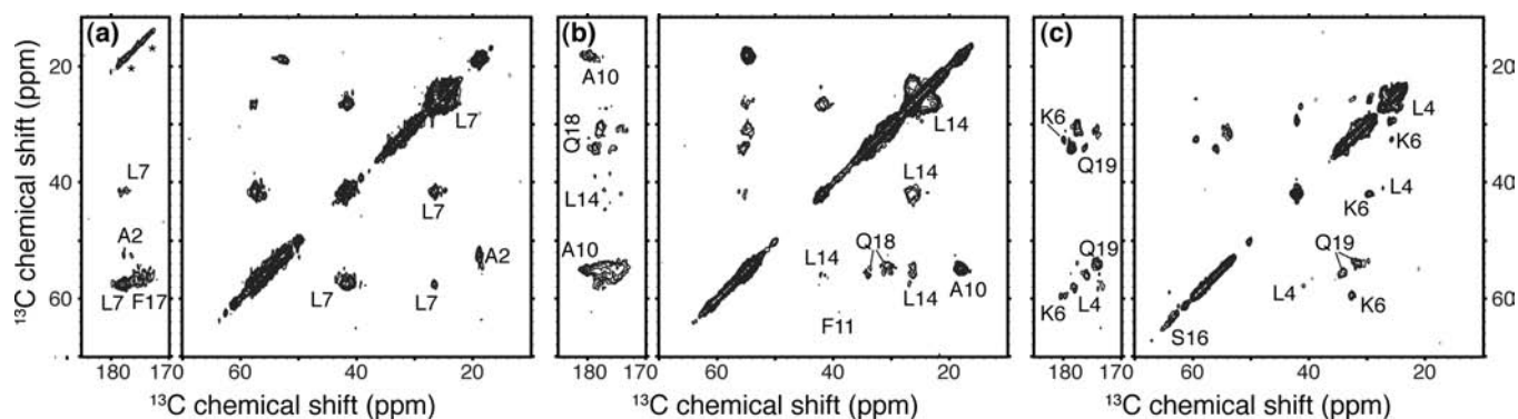
Figure 3. 2D ^{13}\text{C} – ^{13}\text{C} ssNMR spectra using 25 ms DARR mixing, providing 1–2 bond transfers. Measurements on samples p1–p3 are shown in (a)–(c), with (a) obtained at an 800 MHz ^1\text{H} frequency and 16 kHz MAS and (b) and (c) at a 600 MHz ^1\text{H} frequency and 10 and 13 kHz MAS, respectively. Spinning side bands are marked with asterisks. For each spectrum aliphatic-to-carbonyl (left) and intra-aliphatic (right) spectral regions are shown.
